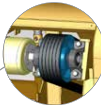
belt transmission with spring tension and safety coupling
